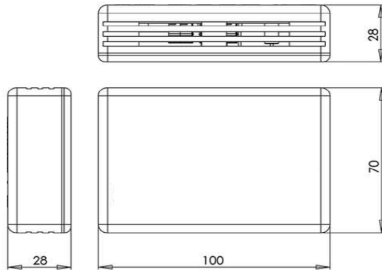
Figure 1.1 IntesisHome® device dimensions in mm
